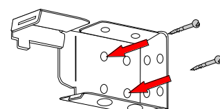
Side fixing: Where the bracket is fixed on to the side wall of a recess.
