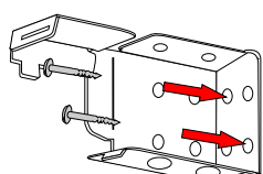
Face fixing: Where the bracket is fixed onto the wall or straight onto the window frame.
